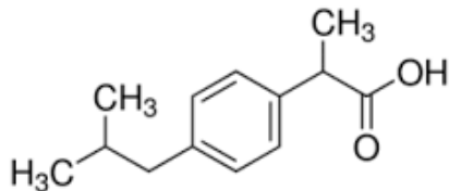
Figure 2: Ibuprofen structure
